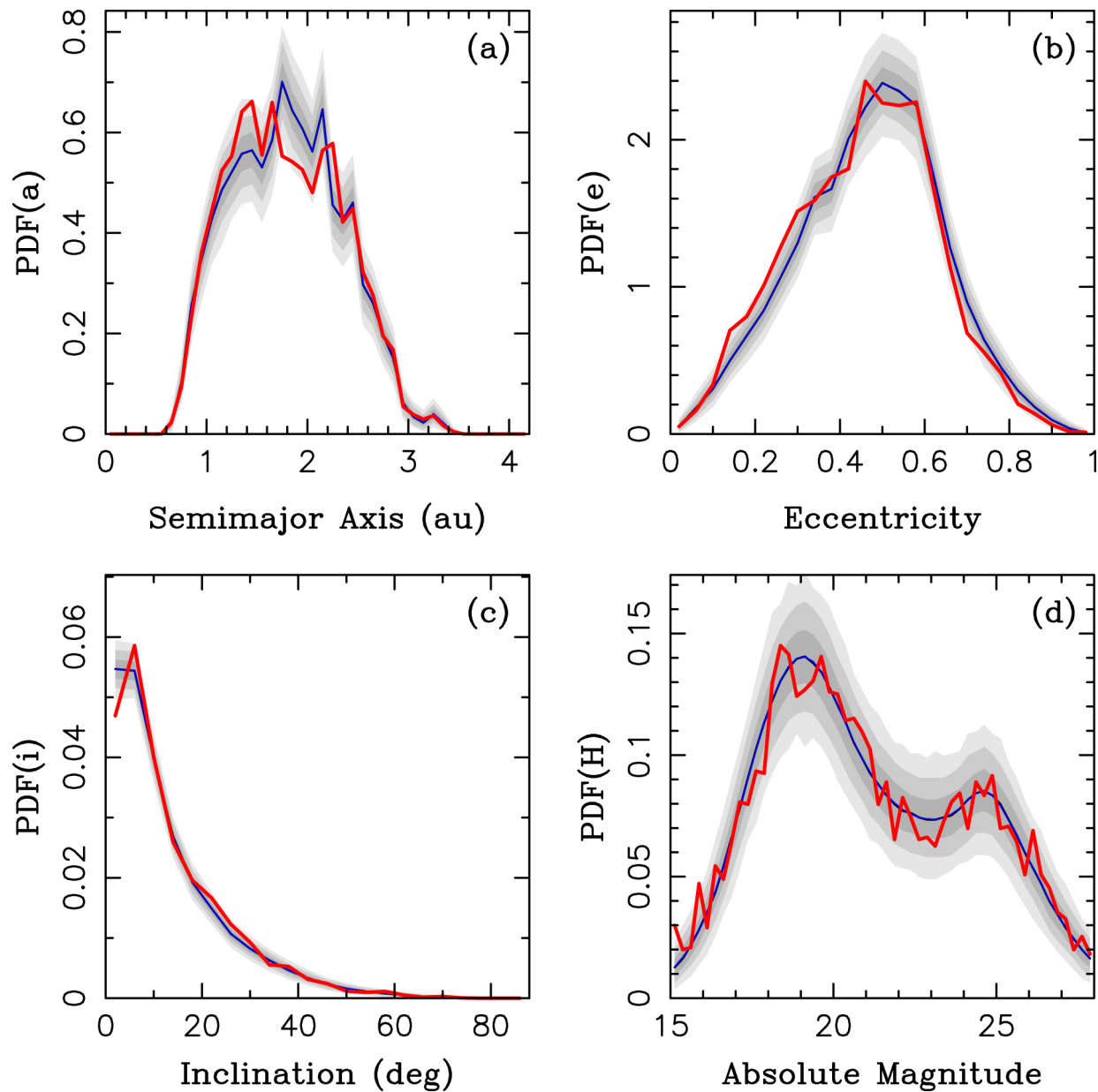
Figure 21. from David Nesvorný et al 2023 Astron. J. 166 doi:10.3847/1538-3881/ace040 https://dx.doi.org/10.3847/1538-3881/ace040 © 2023. The Author(s). Published by the American Astronomical Society.
