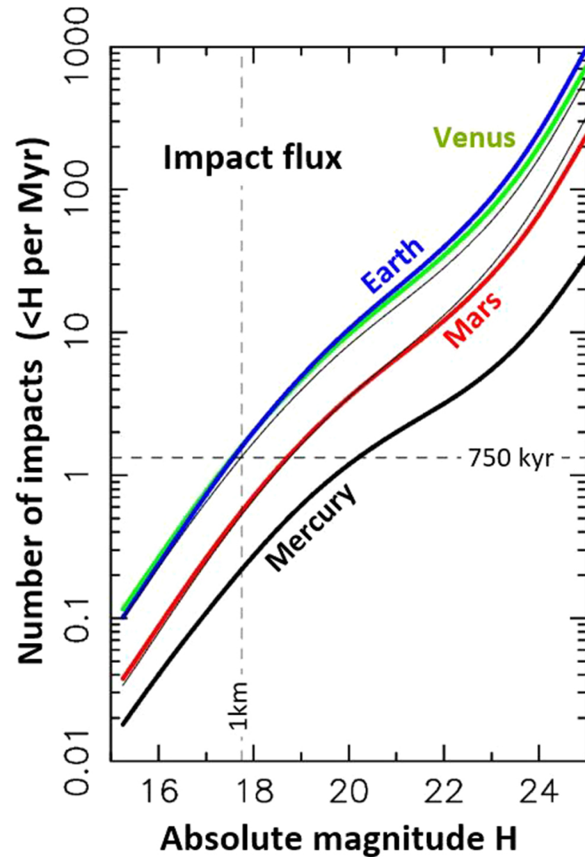
Figure 20. from David Nesvorný et al 2023 Astron. J. 166 doi:10.3847/1538-3881/ace040 https://dx.doi.org/10.3847/1538-3881/ace040 © 2023. The Author(s). Published by the American Astronomical Society.
