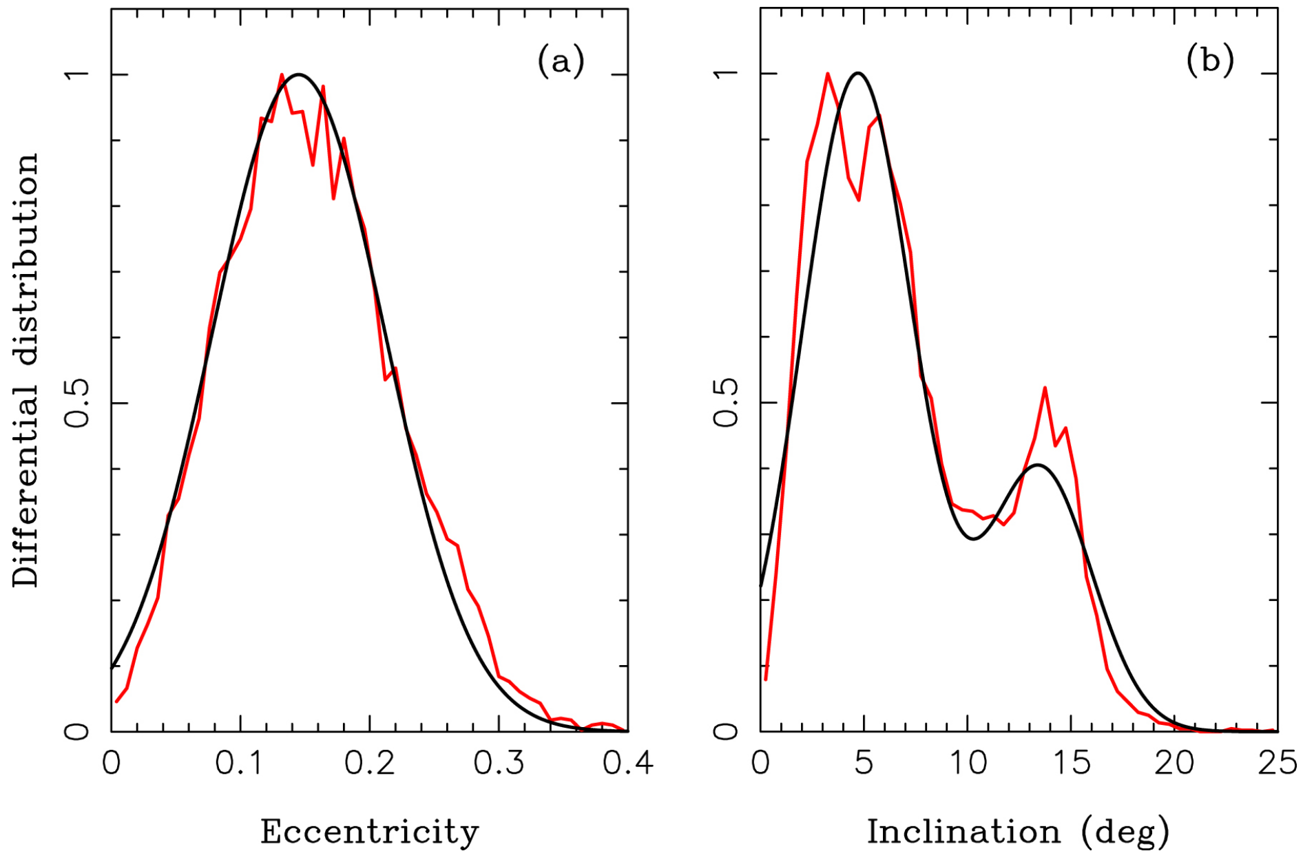
Figure 2. from David Nesvorný et al 2023 Astron. J. 166 doi:10.3847/1538-3881/ace040 https://dx.doi.org/10.3847/1538-3881/ace040 © 2023. The Author(s). Published by the American Astronomical Society.
