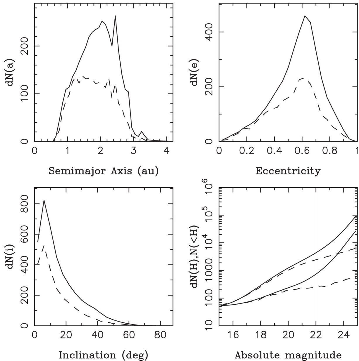
Figure 19. from David Nesvorný et al 2023 Astron. J. 166 doi:10.3847/1538-3881/ace040 https://dx.doi.org/10.3847/1538-3881/ace040 © 2023. The Author(s). Published by the American Astronomical Society.
