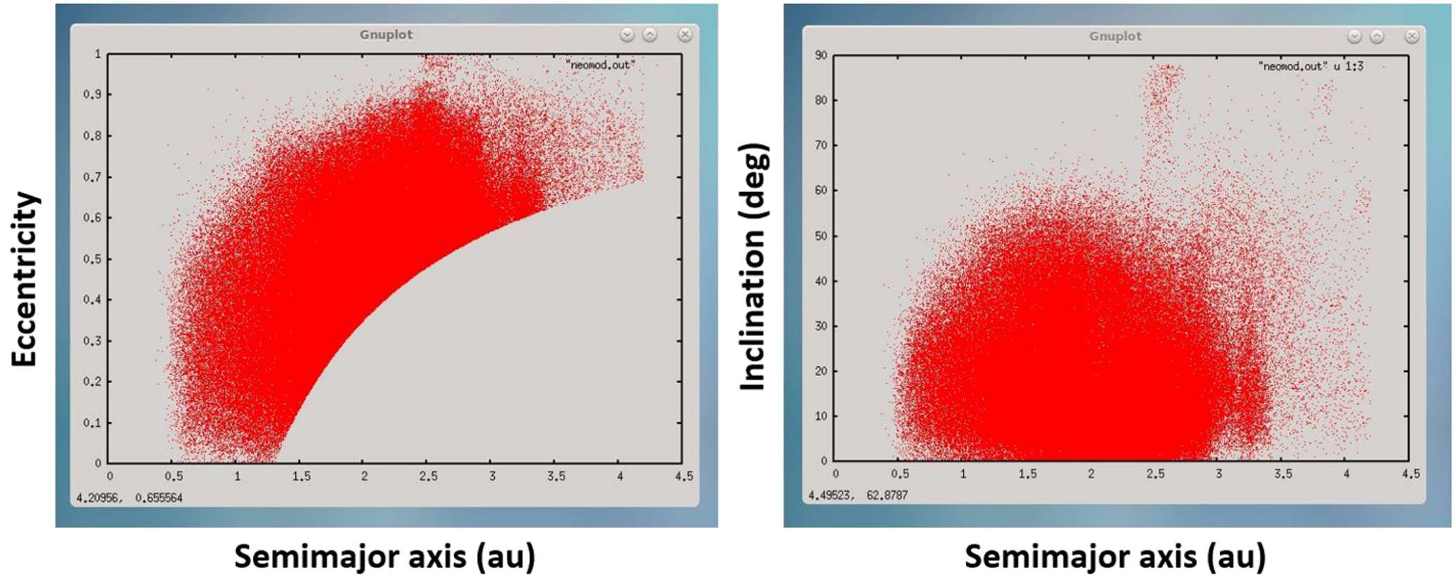
Figure 18. from David Nesvorný et al 2023 Astron. J. 166 doi:10.3847/1538-3881/ace040 https://dx.doi.org/10.3847/1538-3881/ace040 © 2023. The Author(s). Published by the American Astronomical Society.
