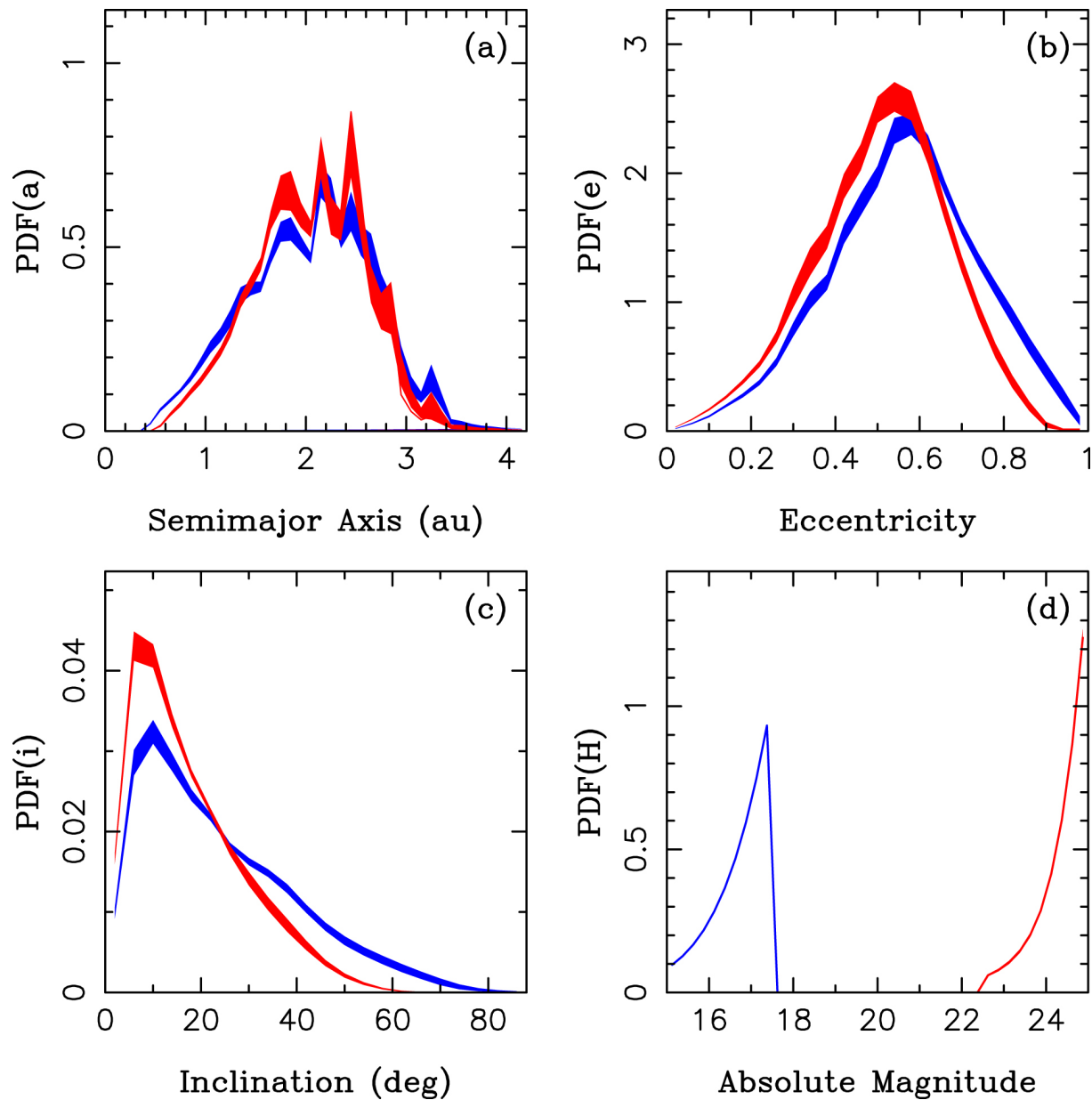
Figure 16. from David Nesvorný et al 2023 Astron. J. 166 doi:10.3847/1538-3881/ace040 https://dx.doi.org/10.3847/1538-3881/ace040 © 2023. The Author(s). Published by the American Astronomical Society.
