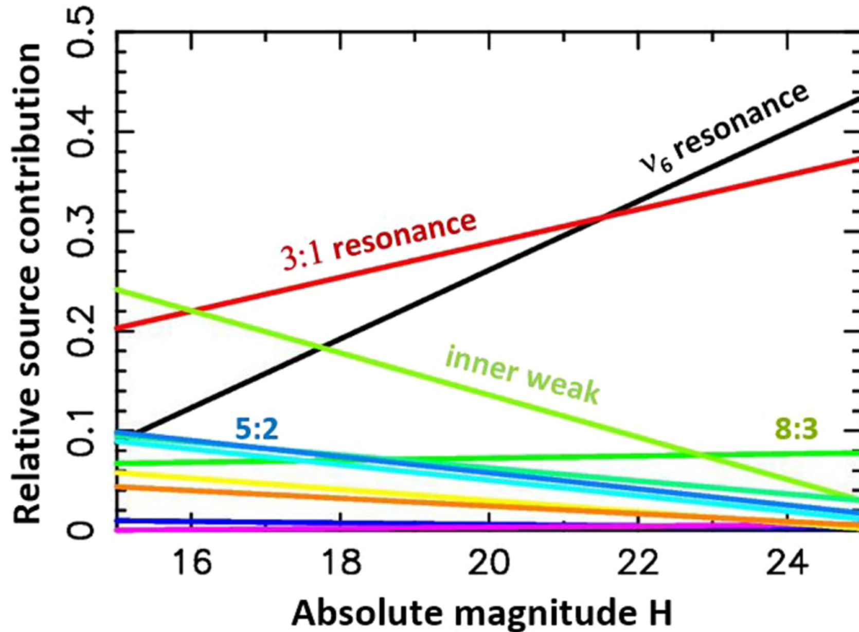
Figure 14. from David Nesvorný et al 2023 Astron. J. 166 doi:10.3847/1538-3881/ace040 https://dx.doi.org/10.3847/1538-3881/ace040 © 2023. The Author(s). Published by the American Astronomical Society.
