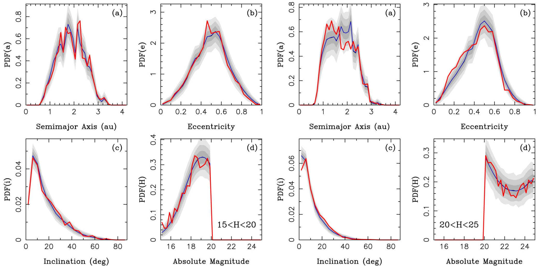
Figure 12. from David Nesvorný et al 2023 Astron. J. 166 doi:10.3847/1538-3881/ace040 https://dx.doi.org/10.3847/1538-3881/ace040 © 2023. The Author(s). Published by the American Astronomical Society.
