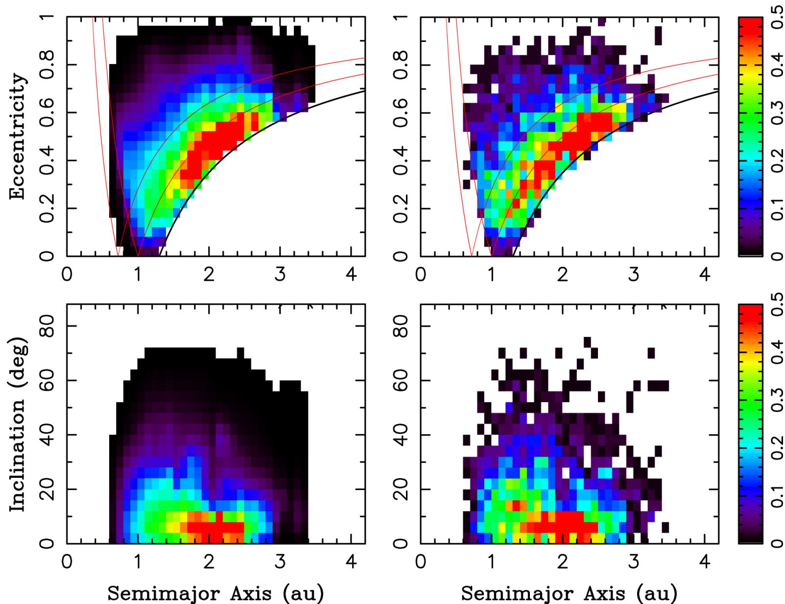
Figure 10. from David Nesvorný et al 2023 Astron. J. 166 doi:10.3847/1538-3881/ace040 https://dx.doi.org/10.3847/1538-3881/ace040 © 2023. The Author(s). Published by the American Astronomical Society.
