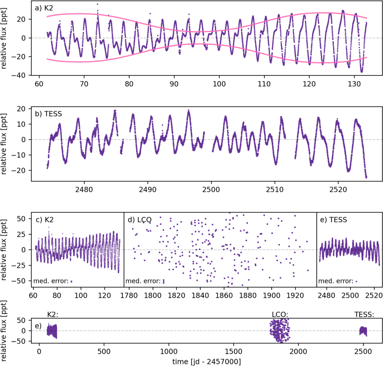
Figure 9. from Sarah Blunt et al 2023 Astron. J. 166 doi:10.3847/1538-3881/acde78 https://dx.doi.org/10.3847/1538-3881/acde78 © 2023. The Author(s). Published by the American Astronomical Society.
