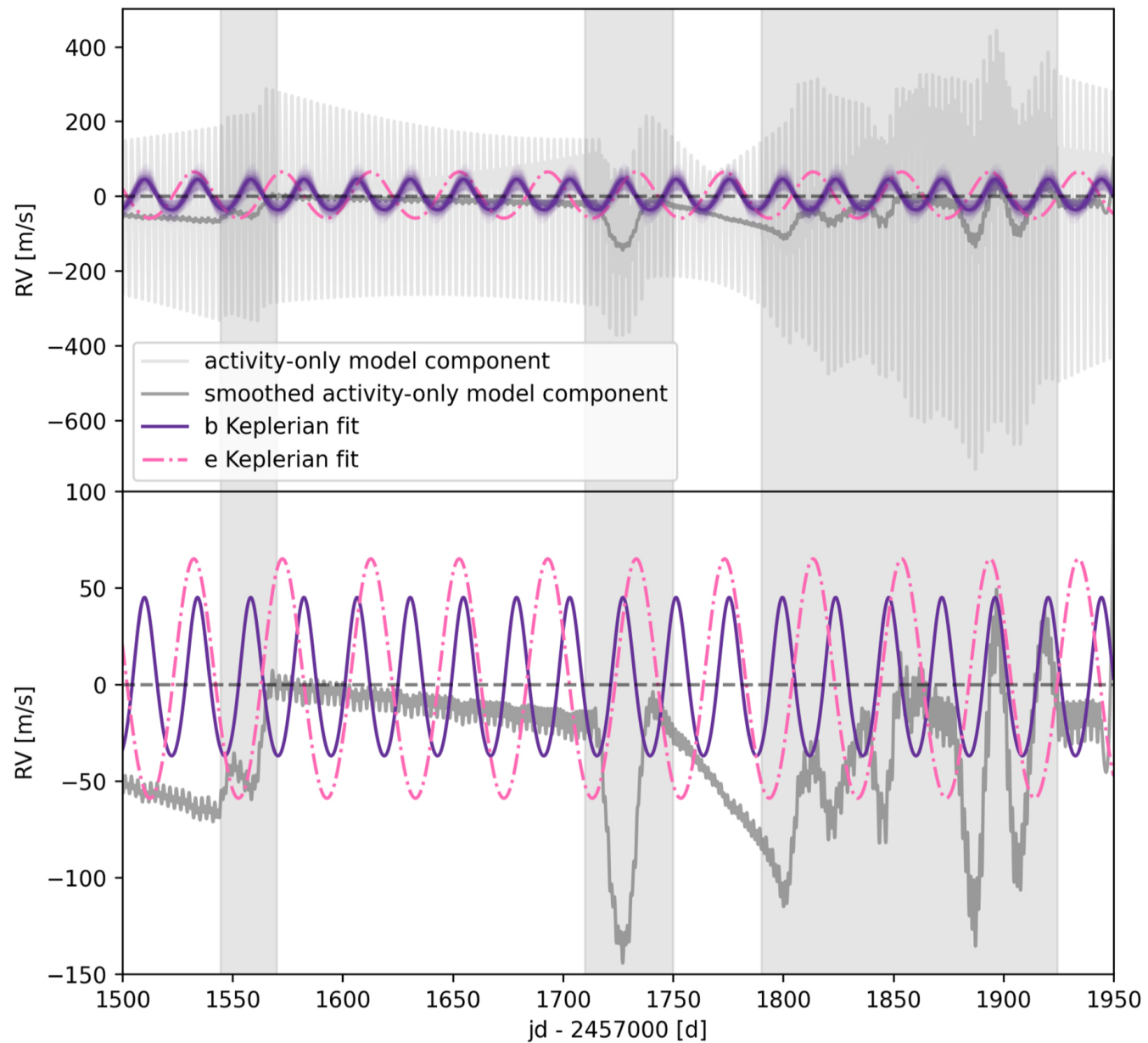
Figure 8. from Sarah Blunt et al 2023 Astron. J. 166 doi:10.3847/1538-3881/acde78 https://dx.doi.org/10.3847/1538-3881/acde78 © 2023. The Author(s). Published by the American Astronomical Society.
