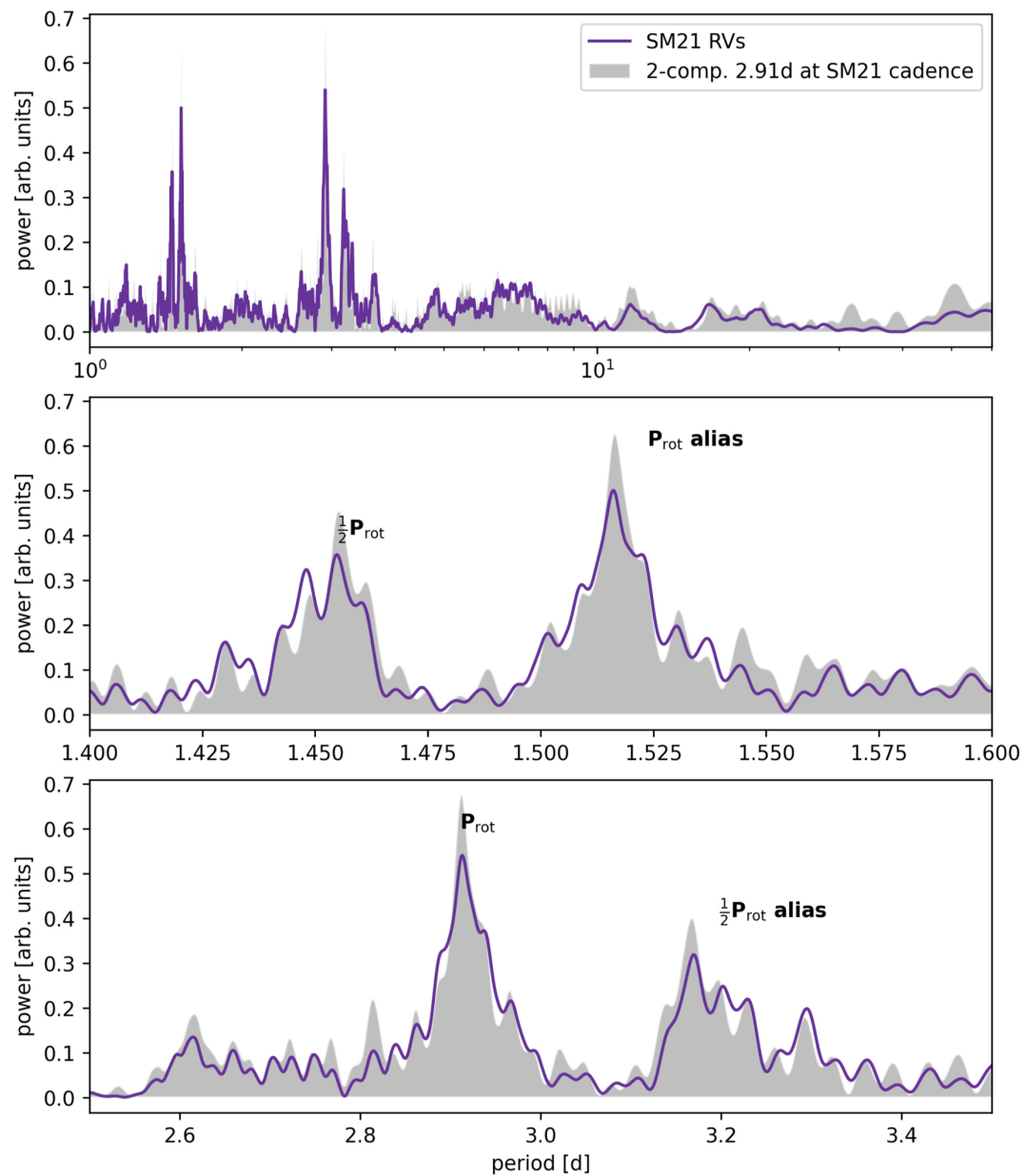
Figure 6. from Sarah Blunt et al 2023 Astron. J. 166 doi:10.3847/1538-3881/acde78 https://dx.doi.org/10.3847/1538-3881/acde78 © 2023. The Author(s). Published by the American Astronomical Society.
