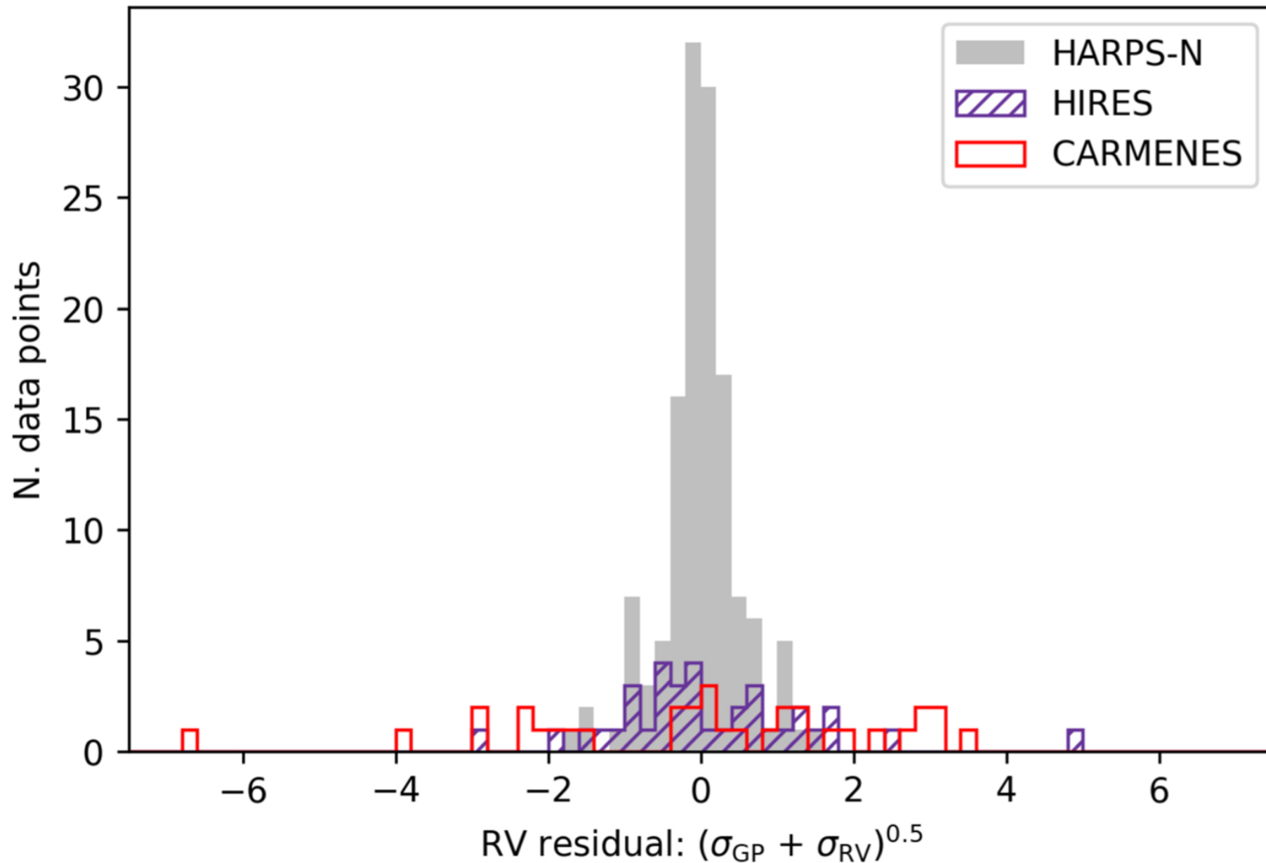
Figure 3. from Sarah Blunt et al 2023 Astron. J. 166 doi:10.3847/1538-3881/acde78 https://dx.doi.org/10.3847/1538-3881/acde78 © 2023. The Author(s). Published by the American Astronomical Society.
