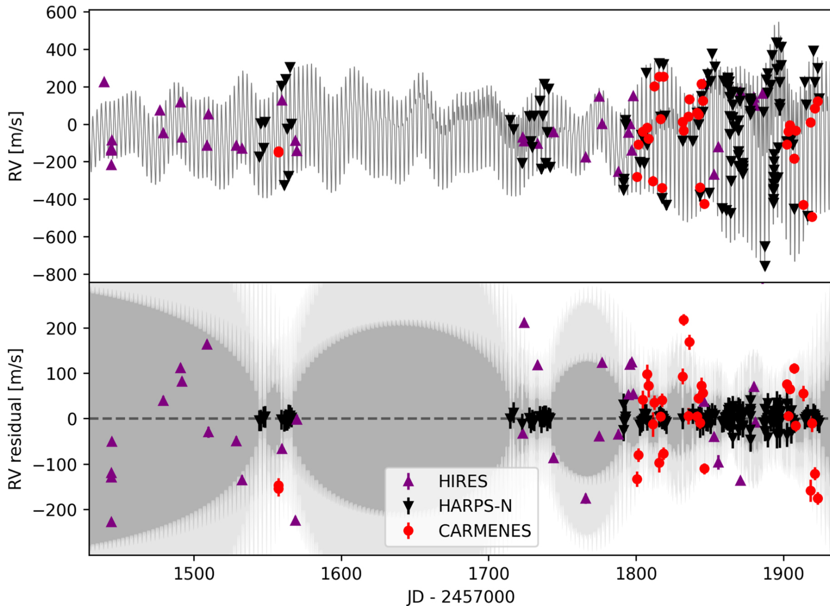
Figure 2. from Sarah Blunt et al 2023 Astron. J. 166 doi:10.3847/1538-3881/acde78 https://dx.doi.org/10.3847/1538-3881/acde78 © 2023. The Author(s). Published by the American Astronomical Society.
