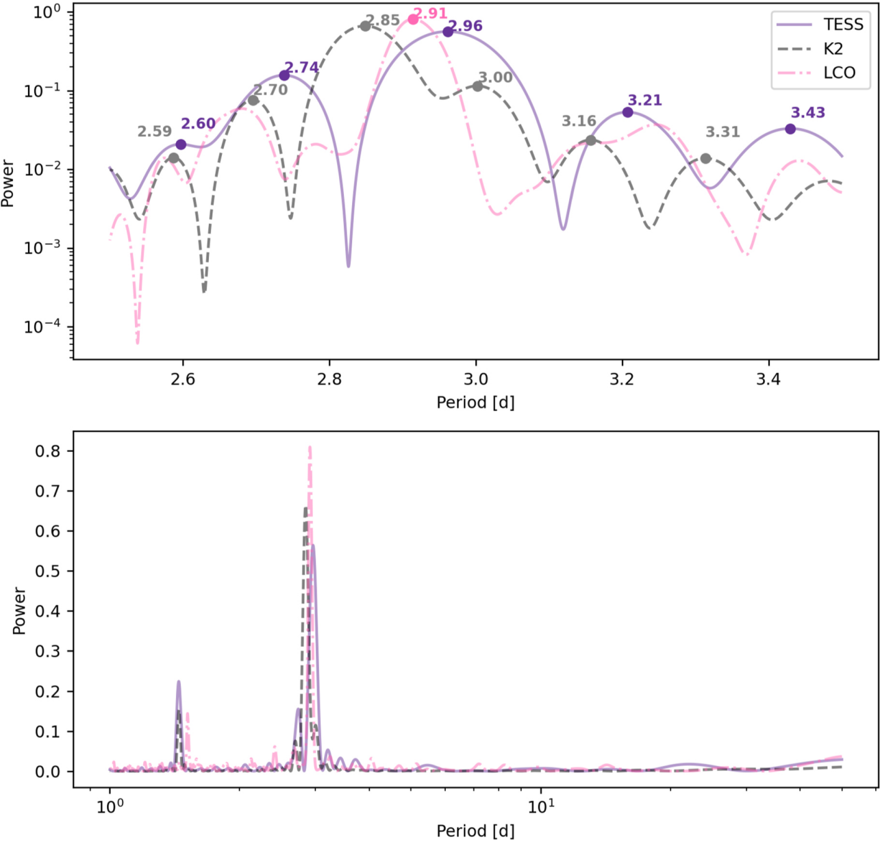
Figure 10. from Sarah Blunt et al 2023 Astron. J. 166 doi:10.3847/1538-3881/acde78 https://dx.doi.org/10.3847/1538-3881/acde78 © 2023. The Author(s). Published by the American Astronomical Society.
