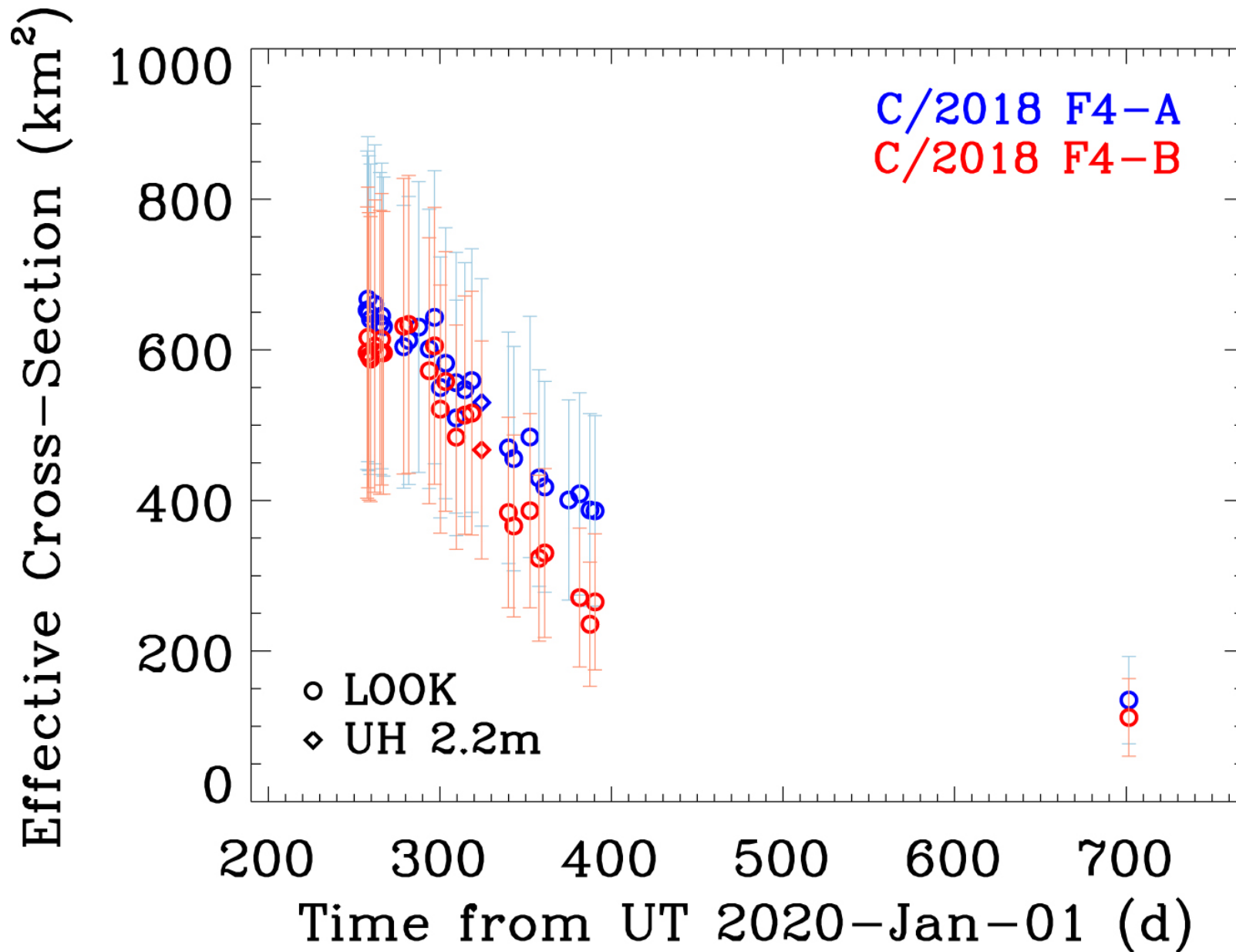
Figure 6. from Man-To Hui et al 2023 Astron. J. 166 doi:10.3847/1538-3881/acdc9c https://dx.doi.org/10.3847/1538-3881/acdc9c © 2023. The Author(s). Published by the American Astronomical Society.
