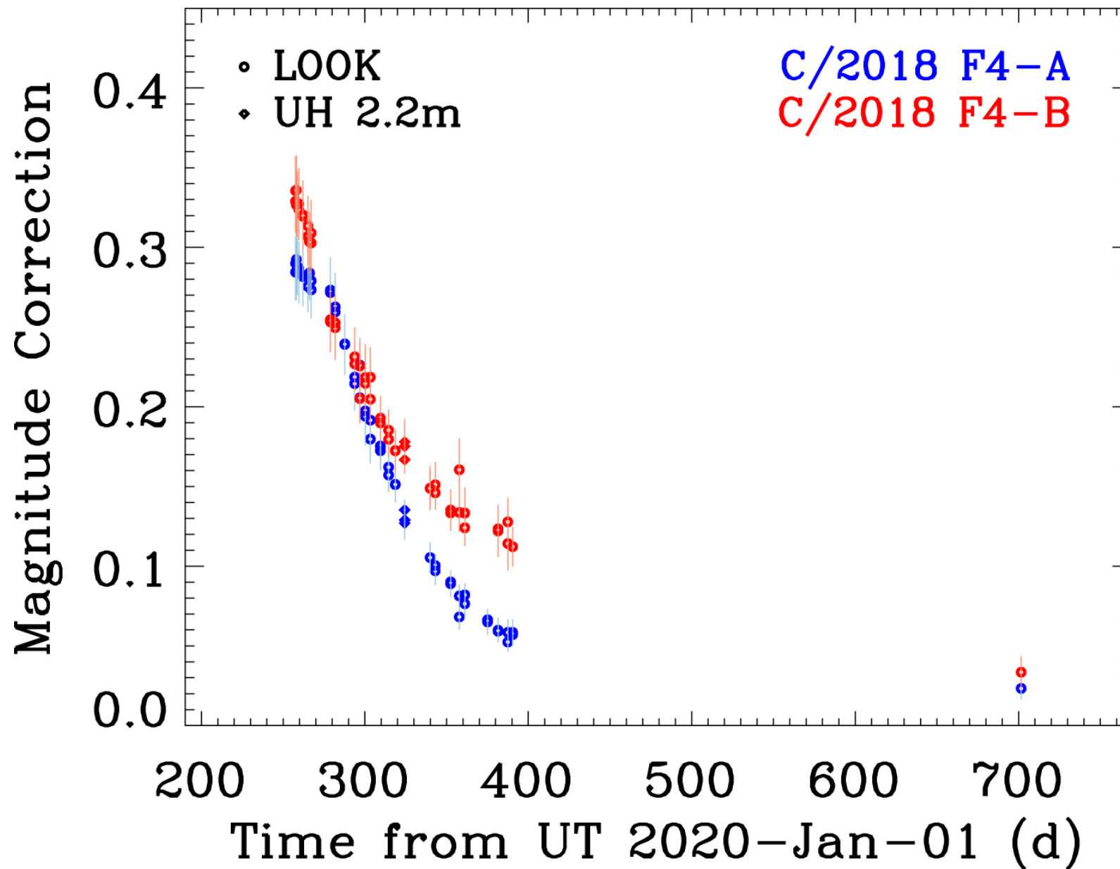
Figure 4. from Man-To Hui et al 2023 Astron. J. 166 doi:10.3847/1538-3881/acdc9c https://dx.doi.org/10.3847/1538-3881/acdc9c © 2023. The Author(s). Published by the American Astronomical Society.
