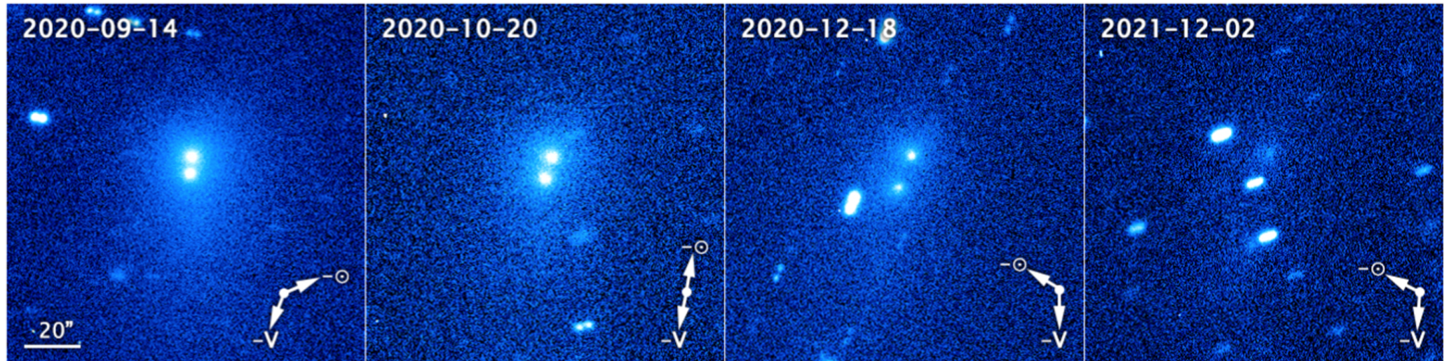
Figure 2. from Man-To Hui et al 2023 Astron. J. 166 doi:10.3847/1538-3881/acdc9c https://dx.doi.org/10.3847/1538-3881/acdc9c © 2023. The Author(s). Published by the American Astronomical Society.
