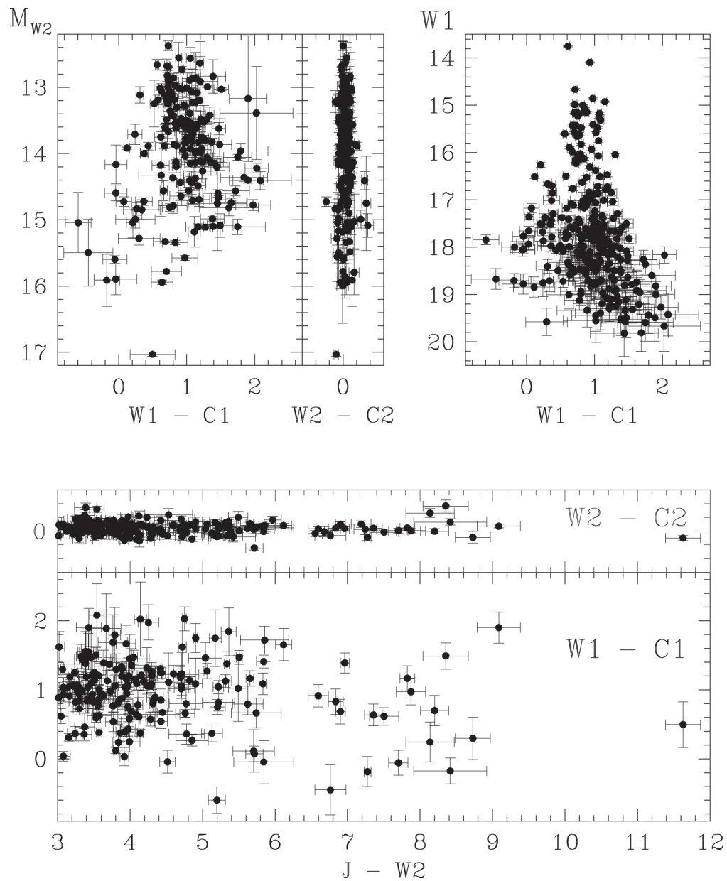
Figure 9. from Aaron M. Meisner et al 2023 Astron. J. 166 doi:10.3847/1538-3881/acdb68 https://dx.doi.org/10.3847/1538-3881/acdb68 © 2023. The Author(s). Published by the American Astronomical Society.
