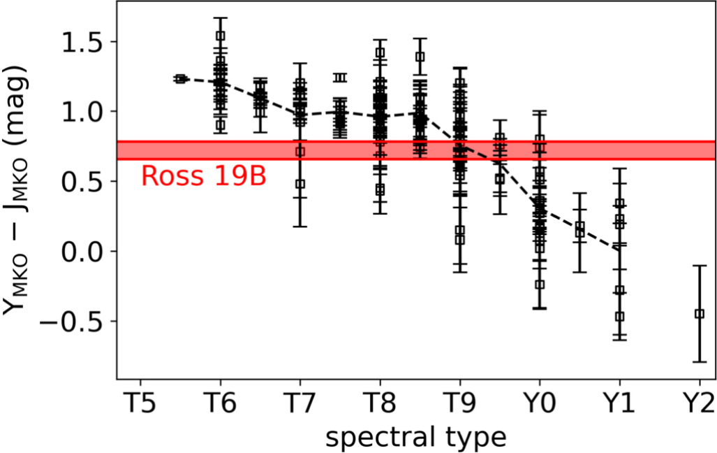
Figure 8. from Aaron M. Meisner et al 2023 Astron. J. 166 doi:10.3847/1538-3881/acdb68 https://dx.doi.org/10.3847/1538-3881/acdb68 © 2023. The Author(s). Published by the American Astronomical Society.
