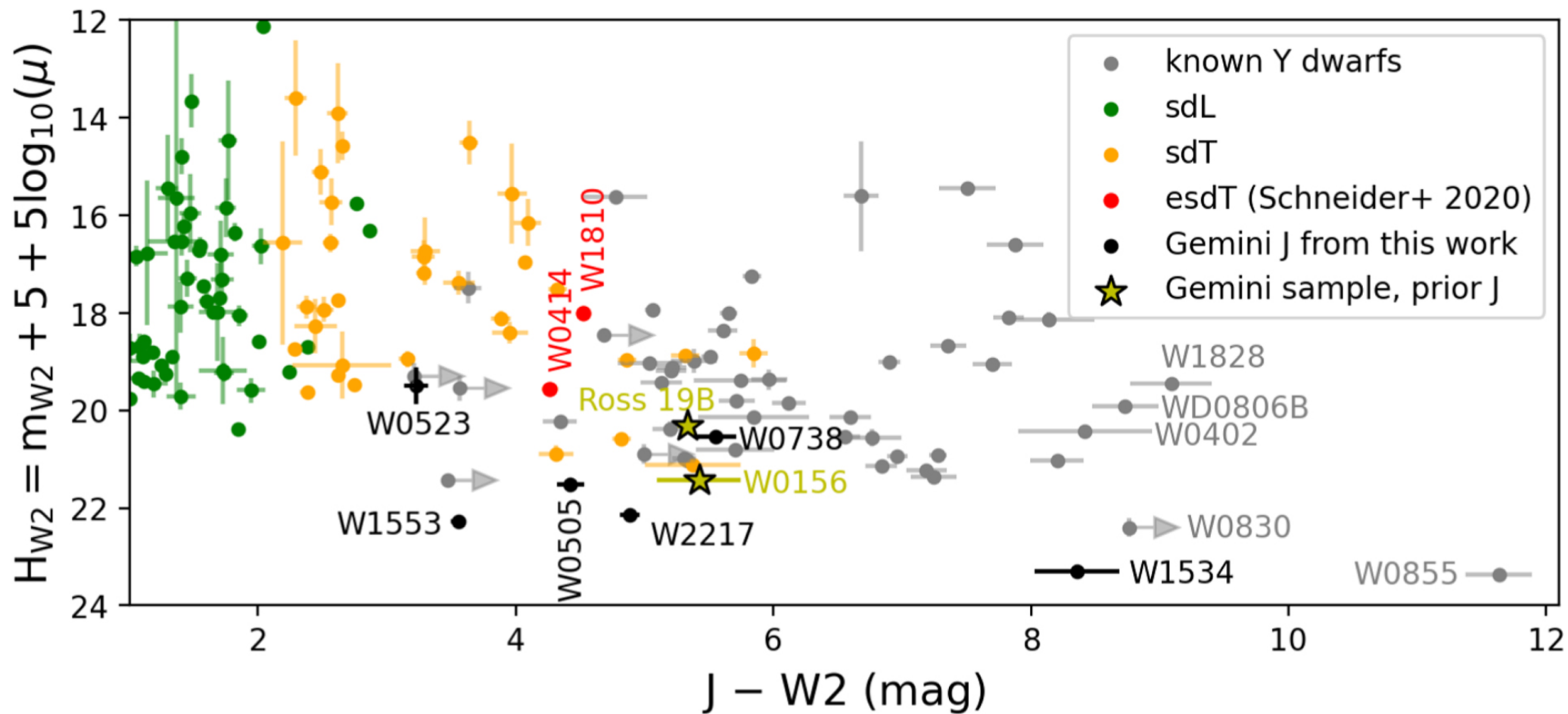
Figure 5. from Aaron M. Meisner et al 2023 Astron. J. 166 doi:10.3847/1538-3881/acdb68 https://dx.doi.org/10.3847/1538-3881/acdb68 © 2023. The Author(s). Published by the American Astronomical Society.
