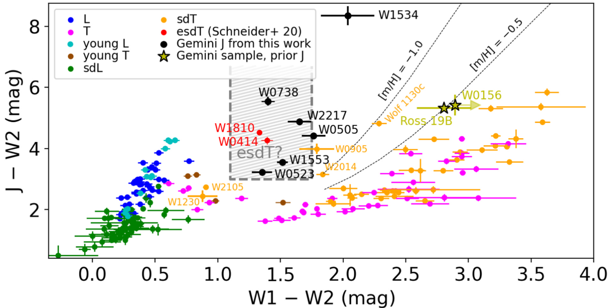
Figure 4. from Aaron M. Meisner et al 2023 Astron. J. 166 doi:10.3847/1538-3881/acdb68 https://dx.doi.org/10.3847/1538-3881/acdb68 © 2023. The Author(s). Published by the American Astronomical Society.
