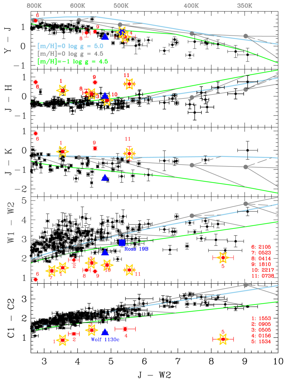
Figure 2. from Aaron M. Meisner et al 2023 Astron. J. 166 doi:10.3847/1538-3881/acdb68 https://dx.doi.org/10.3847/1538-3881/acdb68 © 2023. The Author(s). Published by the American Astronomical Society.
