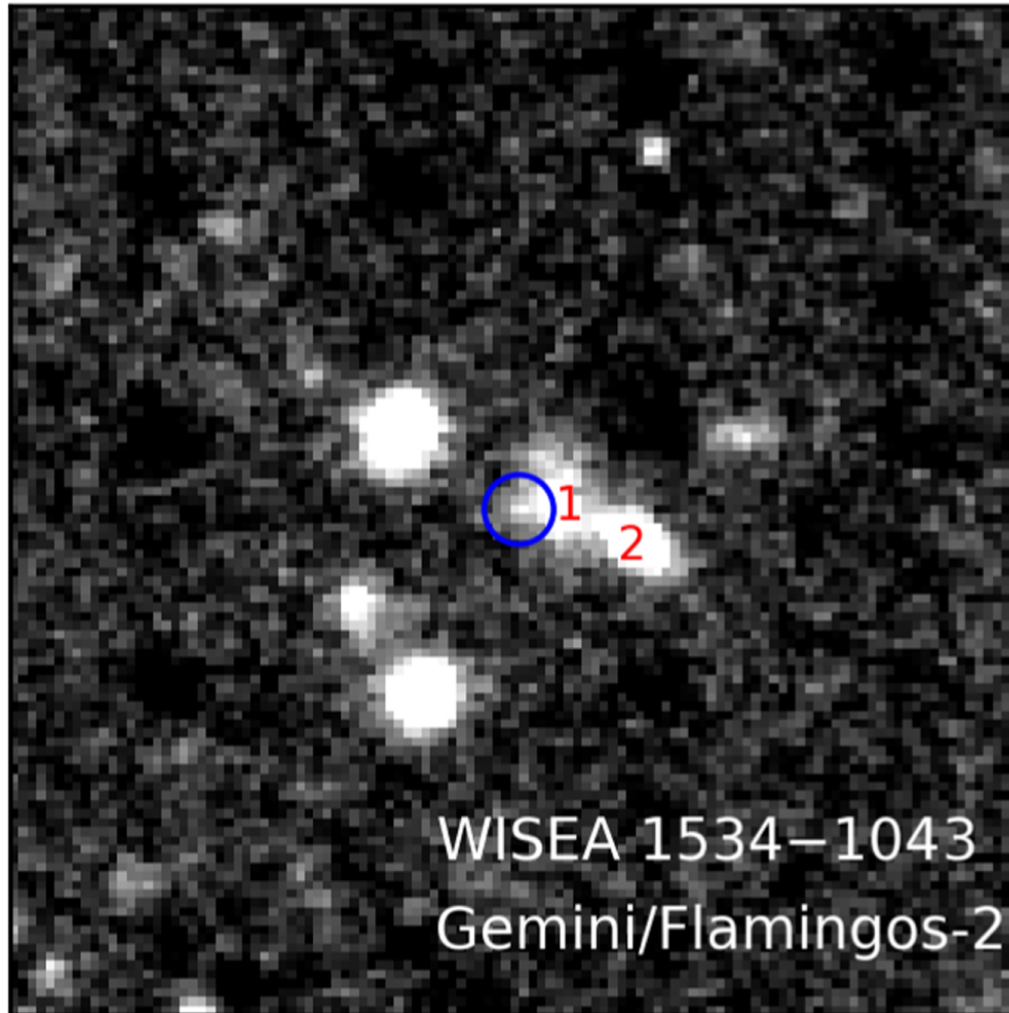
Figure 1. from Aaron M. Meisner et al 2023 Astron. J. 166 doi:10.3847/1538-3881/acdb68 https://dx.doi.org/10.3847/1538-3881/acdb68 © 2023. The Author(s). Published by the American Astronomical Society.
