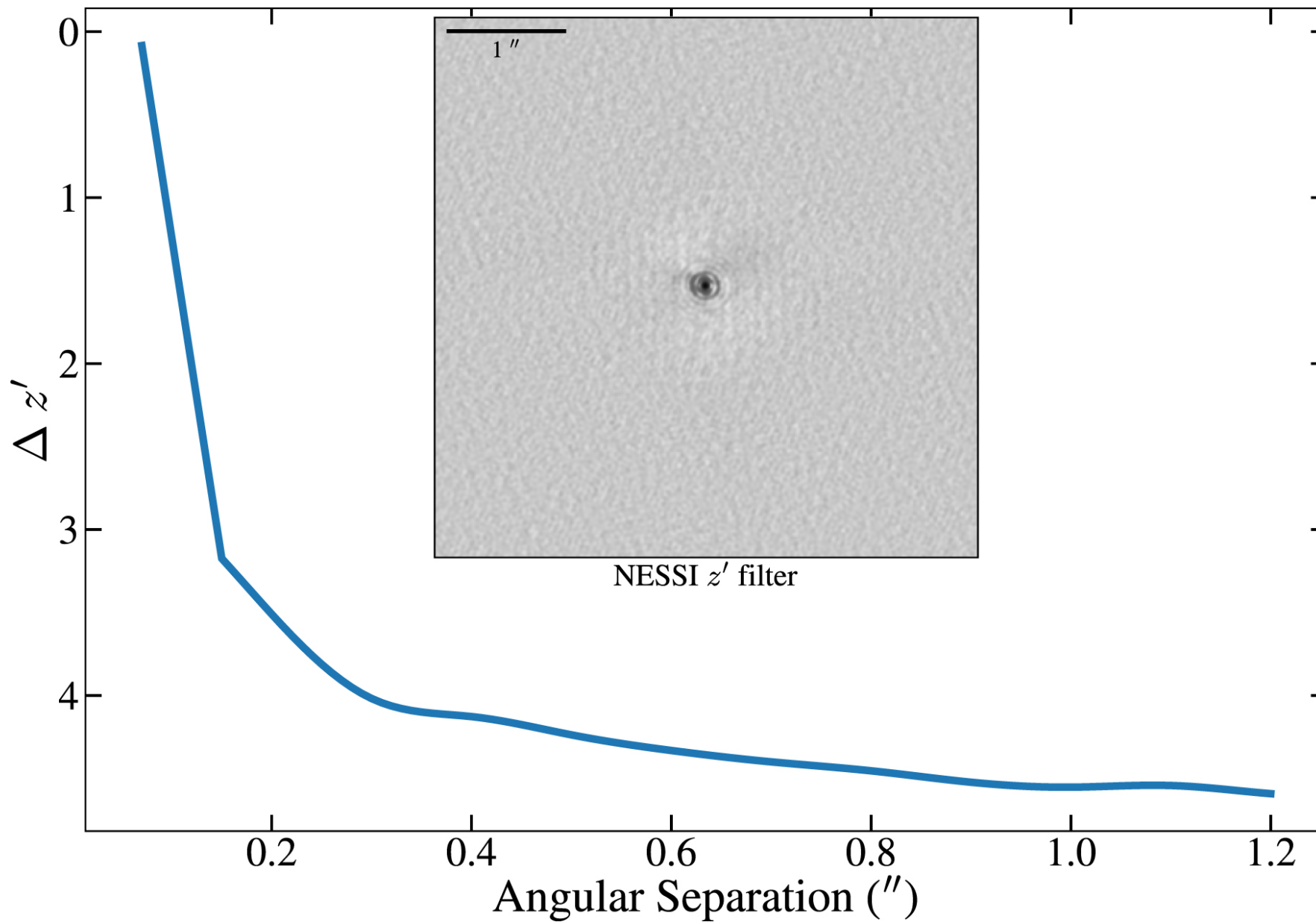
Figure 7. from Caleb I. Cañas et al 2023 Astron. J. 166 doi:10.3847/1538-3881/acdac7 https://dx.doi.org/10.3847/1538-3881/acdac7 © 2023. The Author(s). Published by the American Astronomical Society.
