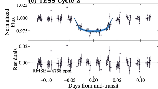
(c) TESS Cycle 2
