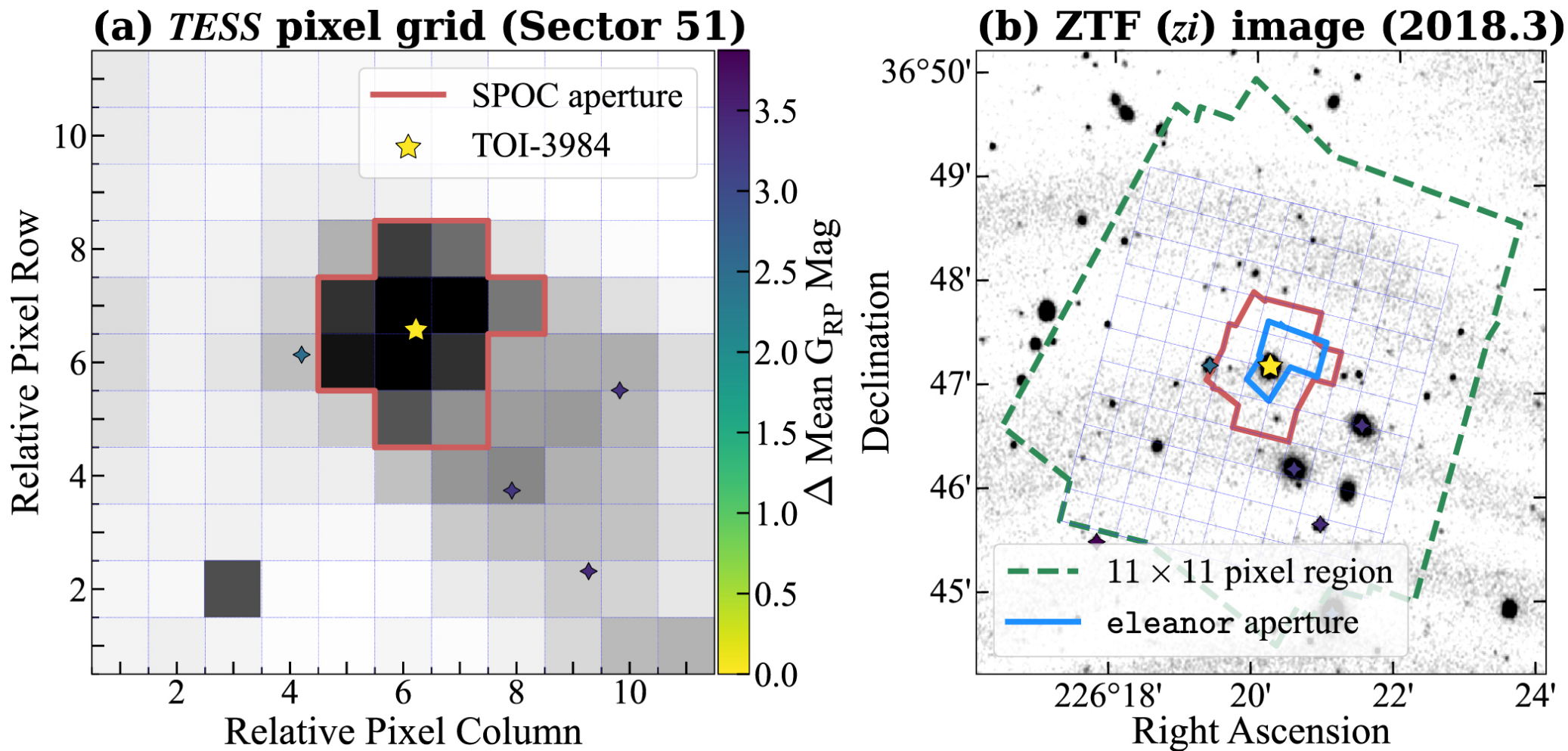
Figure 1. from Caleb I. Cañas et al 2023 Astron. J. 166 doi:10.3847/1538-3881/acdac7 https://dx.doi.org/10.3847/1538-3881/acdac7 © 2023. The Author(s). Published by the American Astronomical Society.
