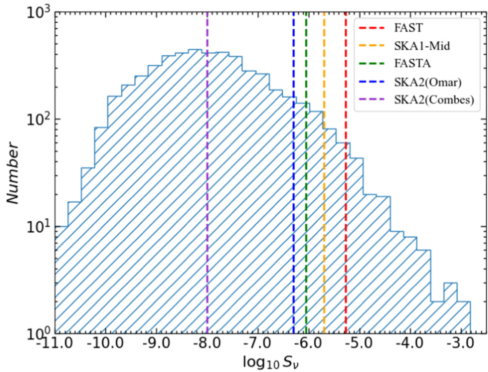
Figure 6. from Qichen Huang et al 2023 Astron. J. 166 doi:10.3847/1538-3881/acd92e https://dx.doi.org/10.3847/1538-3881/acd92e © 2023. The Author(s). Published by the American Astronomical Society.
