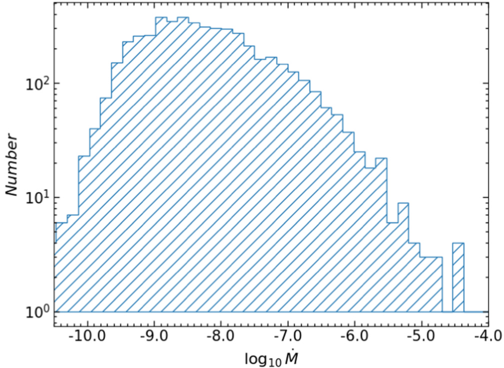
Figure 5. from Qichen Huang et al 2023 Astron. J. 166 doi:10.3847/1538-3881/acd92e https://dx.doi.org/10.3847/1538-3881/acd92e © 2023. The Author(s). Published by the American Astronomical Society.
