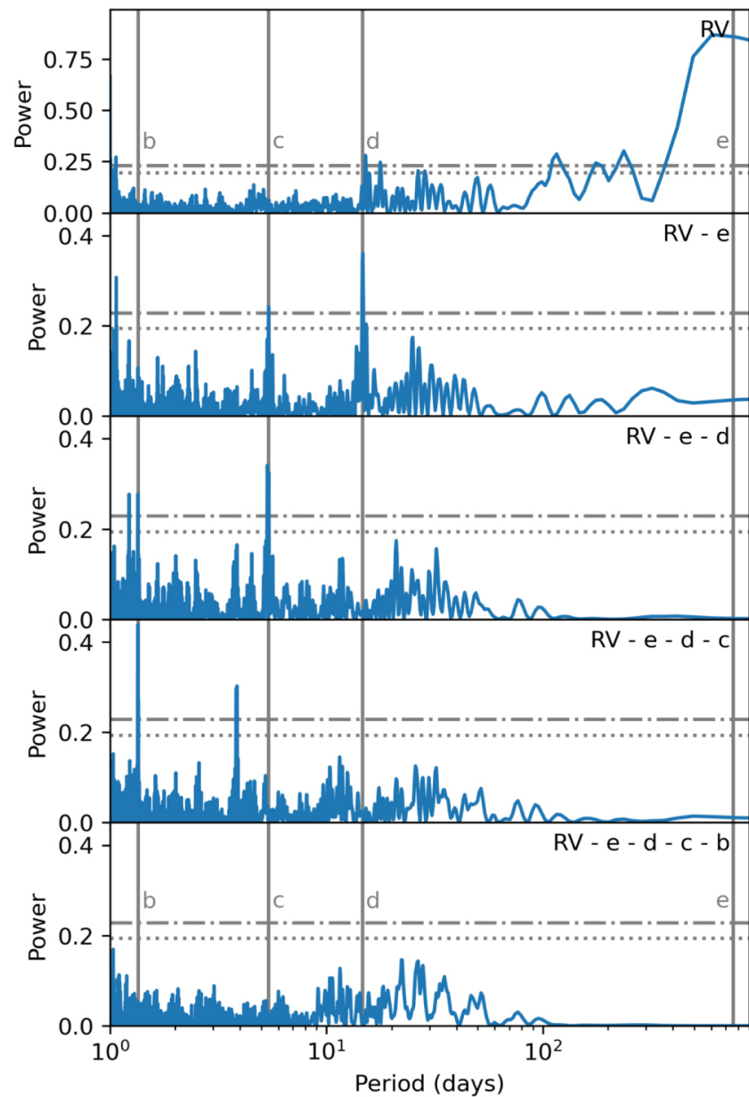
Figure 9. from Michelle Kunimoto et al 2023 Astron. J. 166 doi:10.3847/1538-3881/acd537 https://dx.doi.org/10.3847/1538-3881/acd537 © 2023. The Author(s). Published by the American Astronomical Society.
