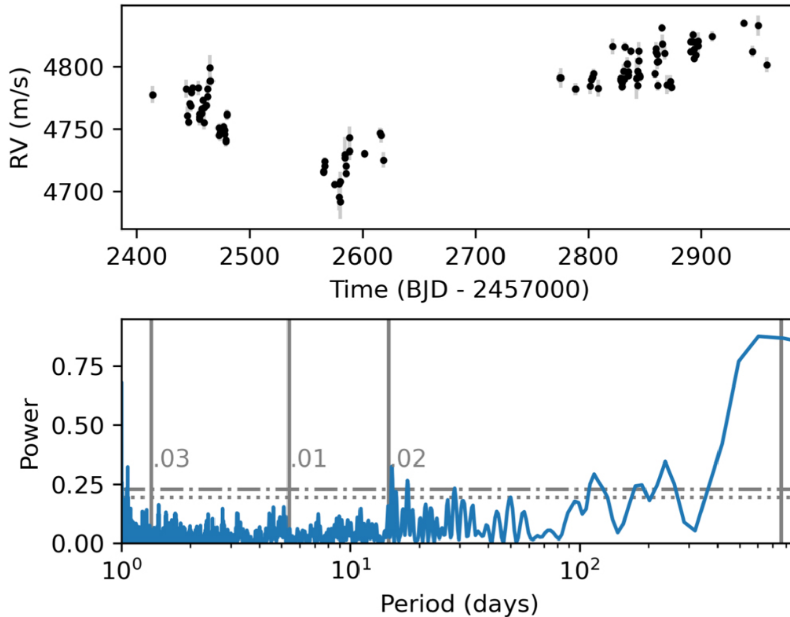
Figure 8. from Michelle Kunimoto et al 2023 Astron. J. 166 doi:10.3847/1538-3881/acd537 https://dx.doi.org/10.3847/1538-3881/acd537 © 2023. The Author(s). Published by the American Astronomical Society.
