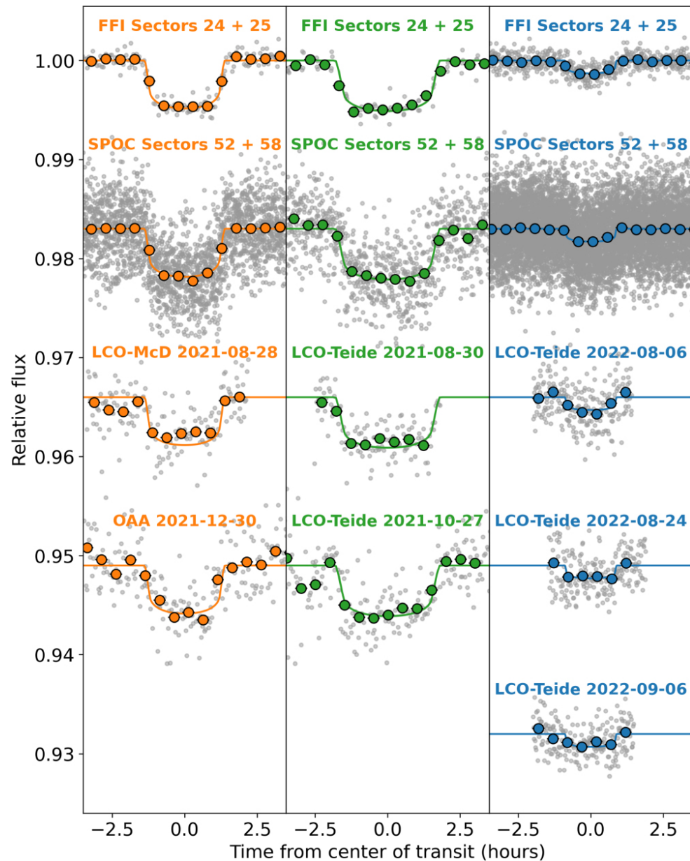
Figure 7. from Michelle Kunimoto et al 2023 Astron. J. 166 doi:10.3847/1538-3881/acd537 https://dx.doi.org/10.3847/1538-3881/acd537 © 2023. The Author(s). Published by the American Astronomical Society.
