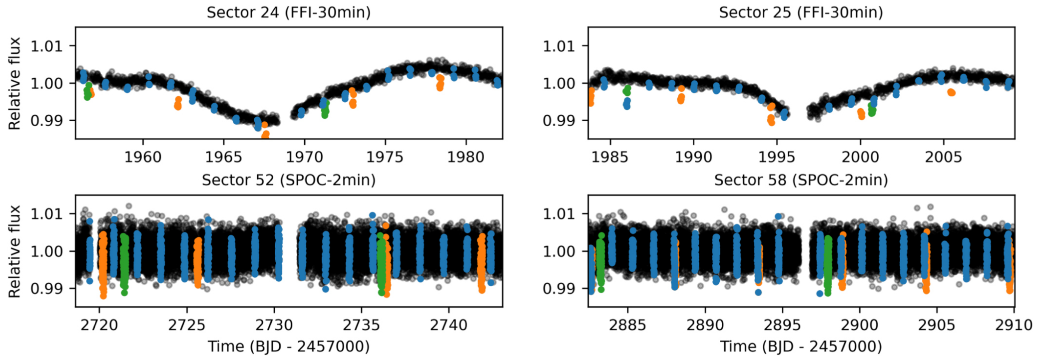
Figure 6. from Michelle Kunimoto et al 2023 Astron. J. 166 doi:10.3847/1538-3881/acd537 https://dx.doi.org/10.3847/1538-3881/acd537 © 2023. The Author(s). Published by the American Astronomical Society.
