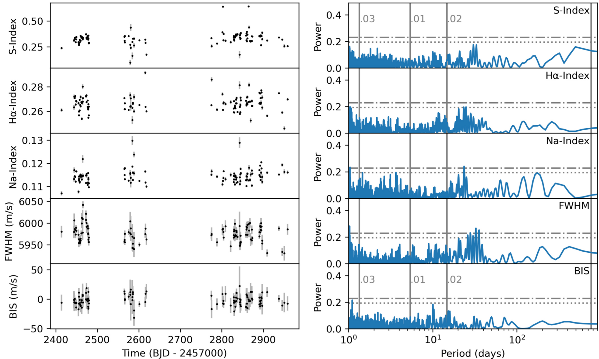
Figure 5. from Michelle Kunimoto et al 2023 Astron. J. 166 doi:10.3847/1538-3881/acd537 https://dx.doi.org/10.3847/1538-3881/acd537 © 2023. The Author(s). Published by the American Astronomical Society.
