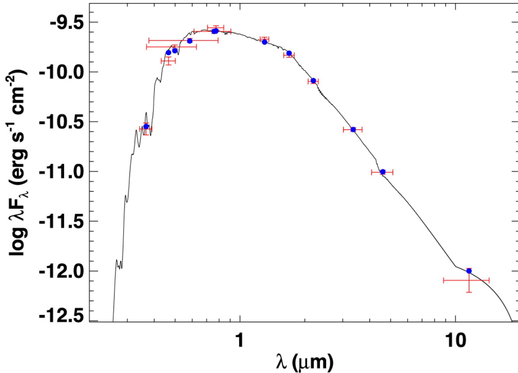
Figure 4. from Michelle Kunimoto et al 2023 Astron. J. 166 doi:10.3847/1538-3881/acd537 https://dx.doi.org/10.3847/1538-3881/acd537 © 2023. The Author(s). Published by the American Astronomical Society.
