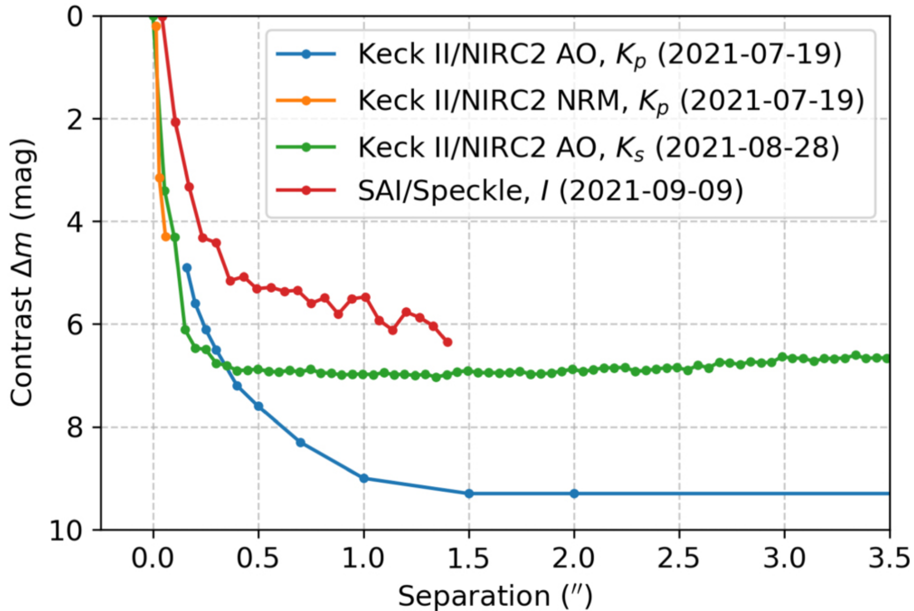
Figure 3. from Michelle Kunimoto et al 2023 Astron. J. 166 doi:10.3847/1538-3881/acd537 https://dx.doi.org/10.3847/1538-3881/acd537 © 2023. The Author(s). Published by the American Astronomical Society.
