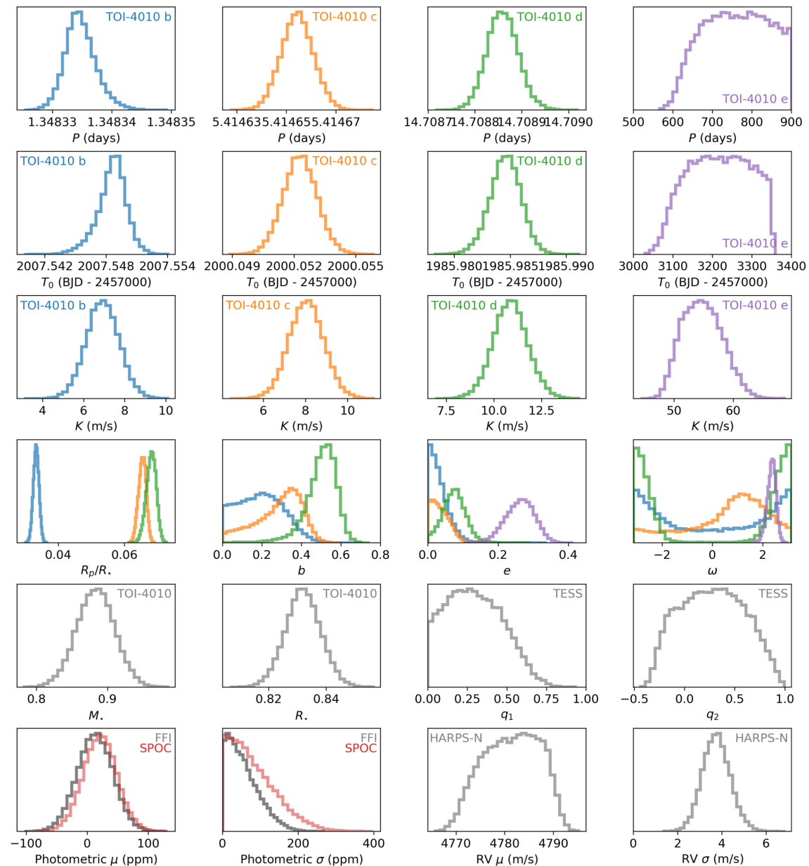
Figure A1. from Michelle Kunimoto et al 2023 Astron. J. 166 doi:10.3847/1538-3881/acd537 https://dx.doi.org/10.3847/1538-3881/acd537 © 2023. The Author(s). Published by the American Astronomical Society.
