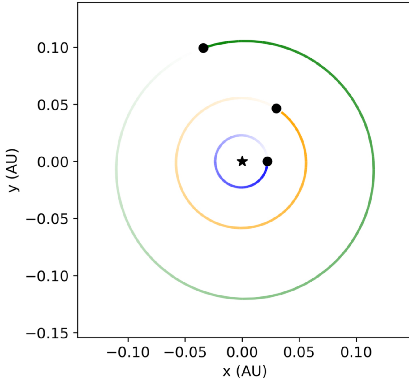
Figure 14. from Michelle Kunimoto et al 2023 Astron. J. 166 doi:10.3847/1538-3881/acd537 https://dx.doi.org/10.3847/1538-3881/acd537 © 2023. The Author(s). Published by the American Astronomical Society.
