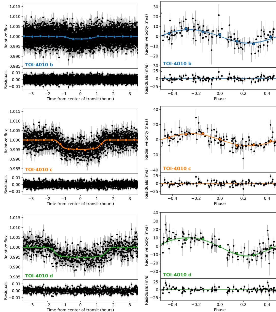
Figure 10. from Michelle Kunimoto et al 2023 Astron. J. 166 doi:10.3847/1538-3881/acd537 https://dx.doi.org/10.3847/1538-3881/acd537 © 2023. The Author(s). Published by the American Astronomical Society.
