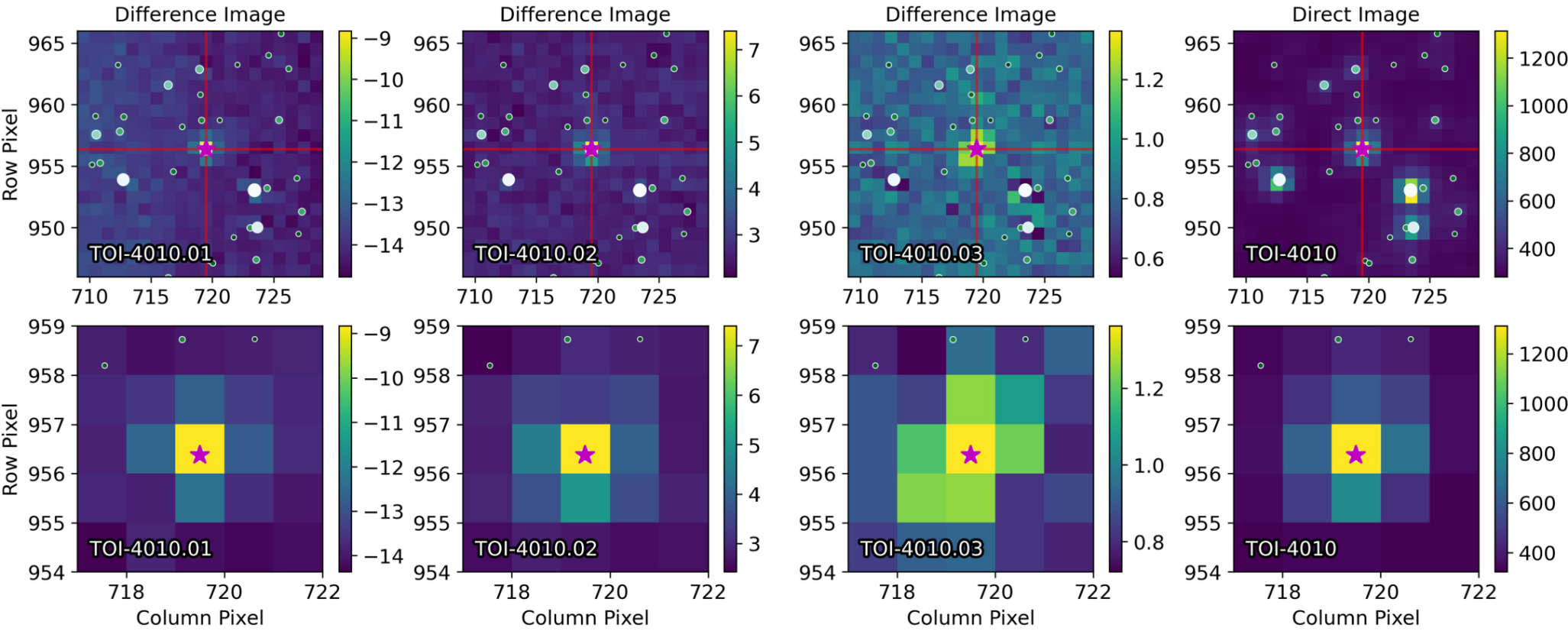
Figure 1. from Michelle Kunimoto et al 2023 Astron. J. 166 doi:10.3847/1538-3881/acd537 https://dx.doi.org/10.3847/1538-3881/acd537 © 2023. The Author(s). Published by the American Astronomical Society.
