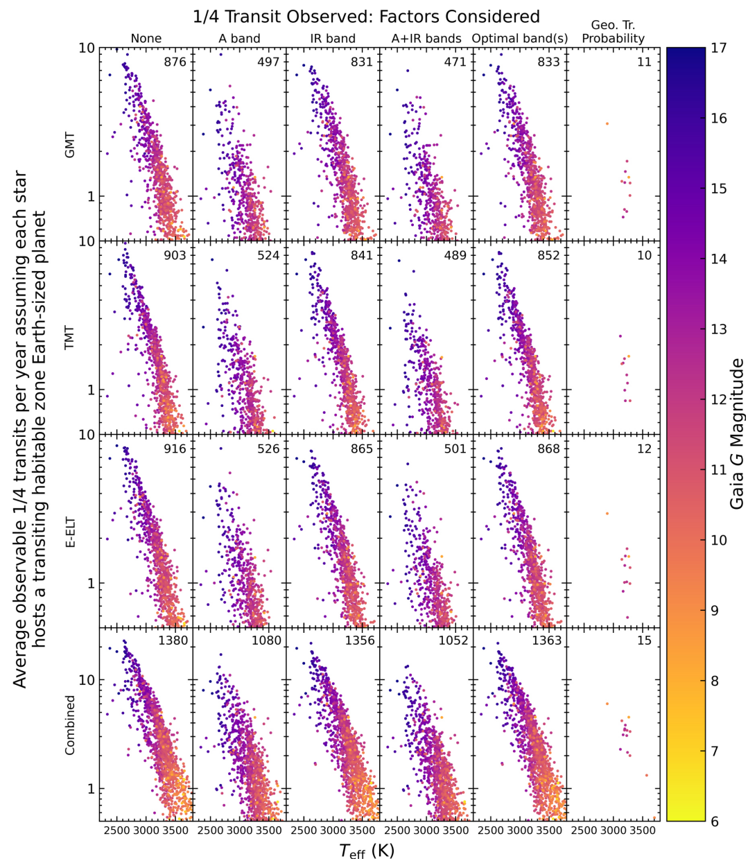
Figure 8. from Kevin K. Hardegree-Ullman et al 2023 Astron. J. 165 doi:10.3847/1538-3881/acd1ec https://dx.doi.org/10.3847/1538-3881/acd1ec © 2023. The Author(s). Published by the American Astronomical Society.
