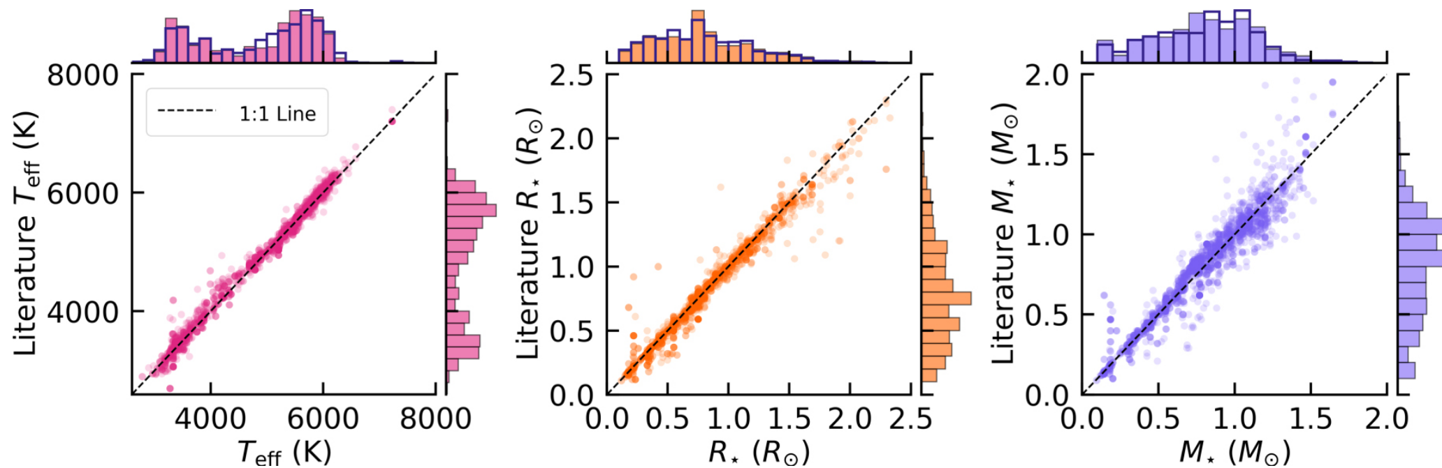
Figure 4. from Kevin K. Hardegree-Ullman et al 2023 Astron. J. 165 doi:10.3847/1538-3881/acd1ec https://dx.doi.org/10.3847/1538-3881/acd1ec © 2023. The Author(s). Published by the American Astronomical Society.
