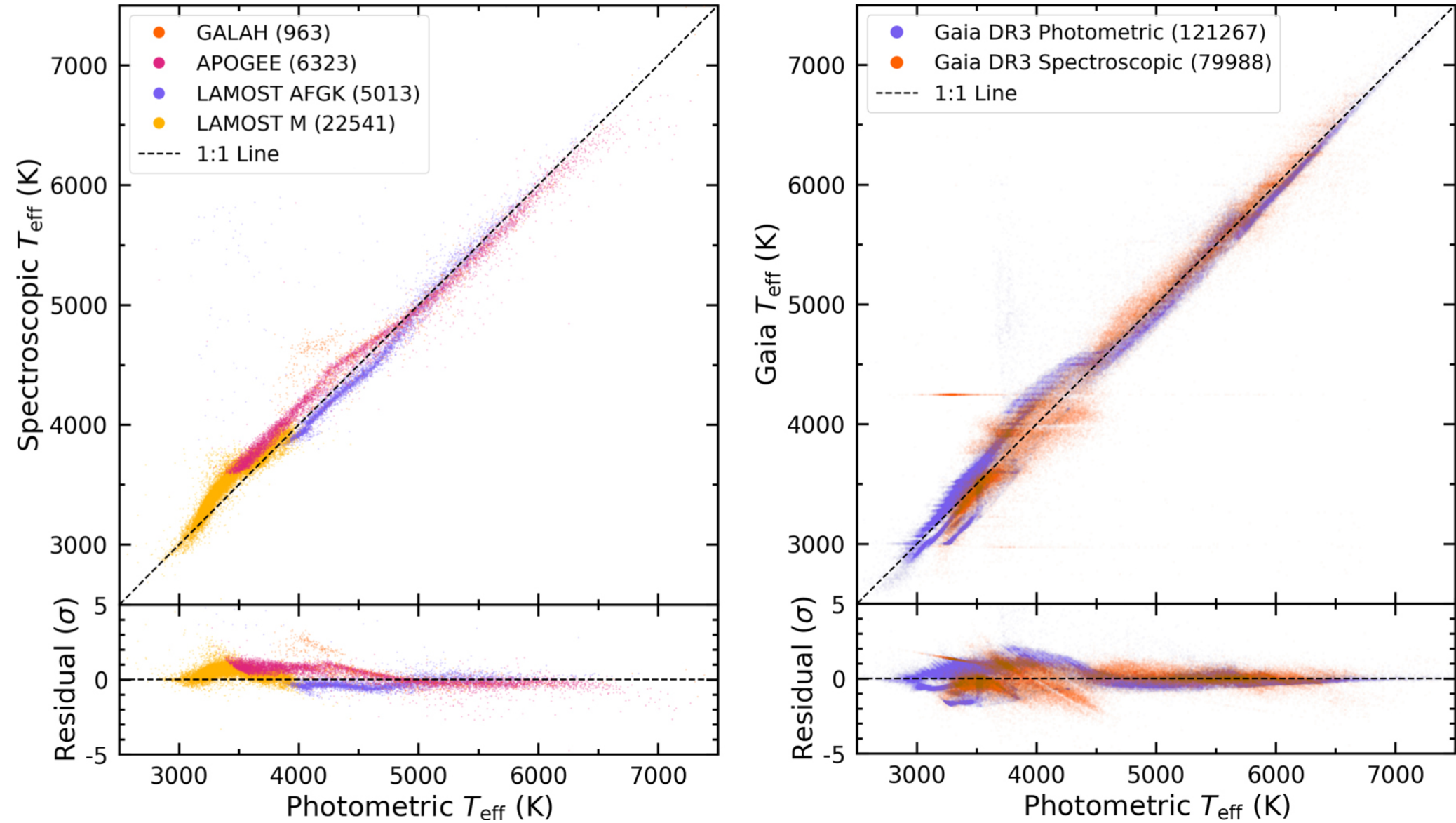
Figure 3. from Kevin K. Hardegree-Ullman et al 2023 Astron. J. 165 doi:10.3847/1538-3881/acd1ec https://dx.doi.org/10.3847/1538-3881/acd1ec © 2023. The Author(s). Published by the American Astronomical Society.
