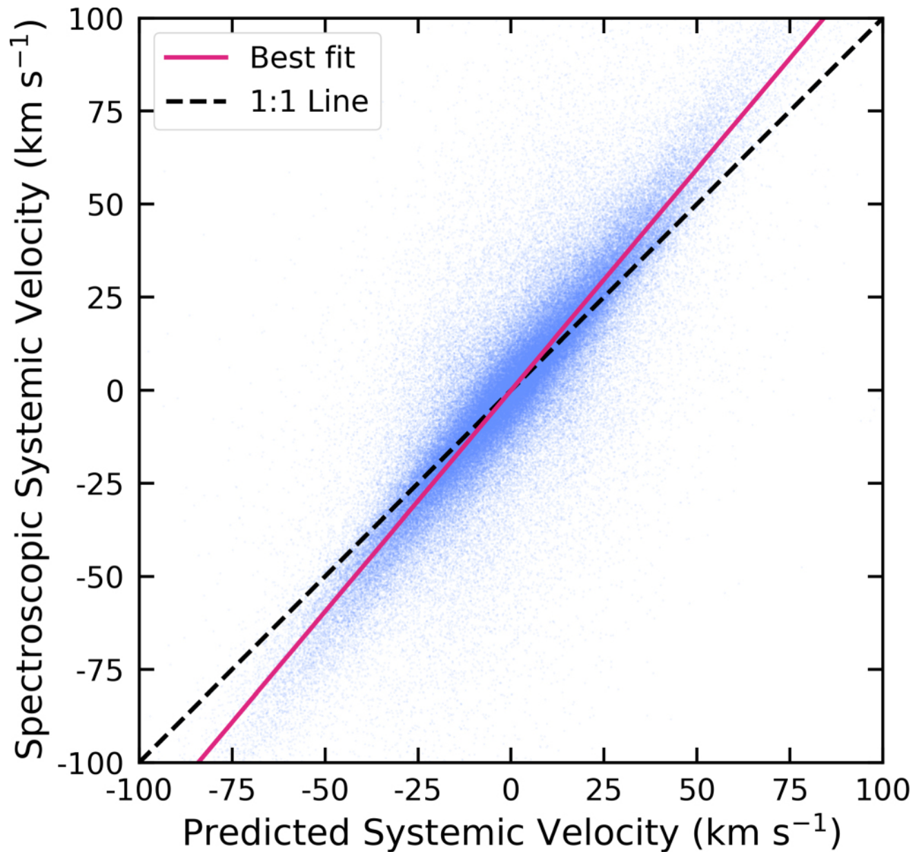
Figure 2. from Kevin K. Hardegree-Ullman et al 2023 Astron. J. 165 doi:10.3847/1538-3881/acd1ec https://dx.doi.org/10.3847/1538-3881/acd1ec © 2023. The Author(s). Published by the American Astronomical Society.
