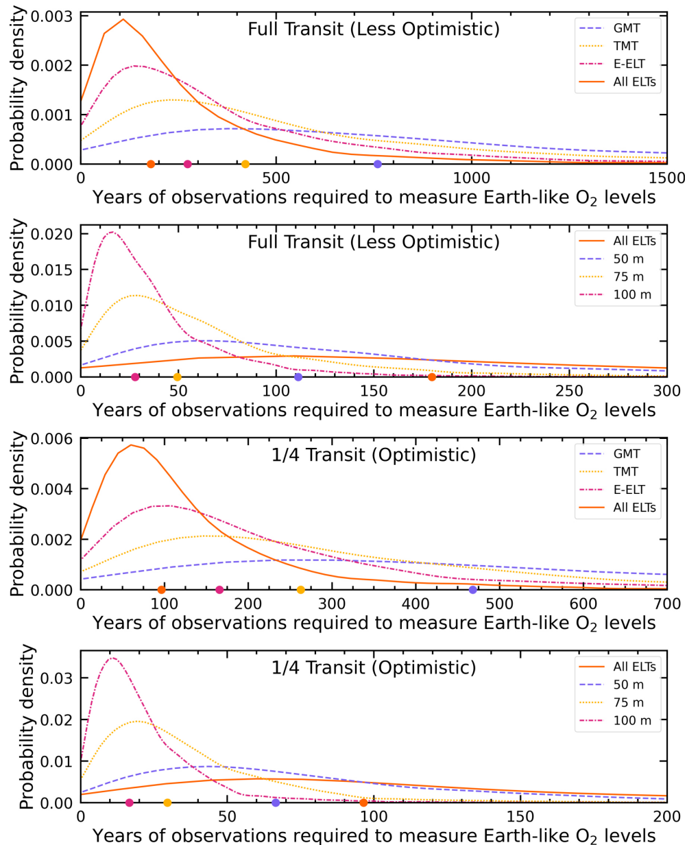
Figure 10. from Kevin K. Hardegree-Ullman et al 2023 Astron. J. 165 doi:10.3847/1538-3881/acd1ec https://dx.doi.org/10.3847/1538-3881/acd1ec © 2023. The Author(s). Published by the American Astronomical Society.
