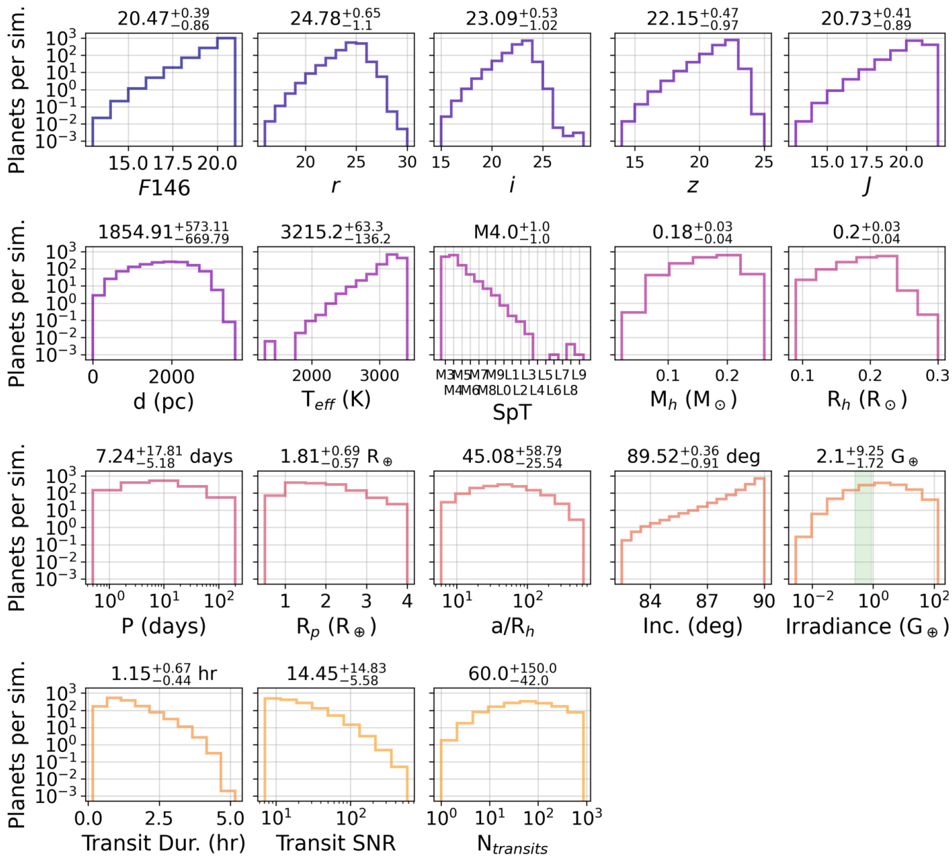
Figure 9. from Patrick Tamburo et al 2023 Astron. J. 165 doi:10.3847/1538-3881/acd1de https://dx.doi.org/10.3847/1538-3881/acd1de
