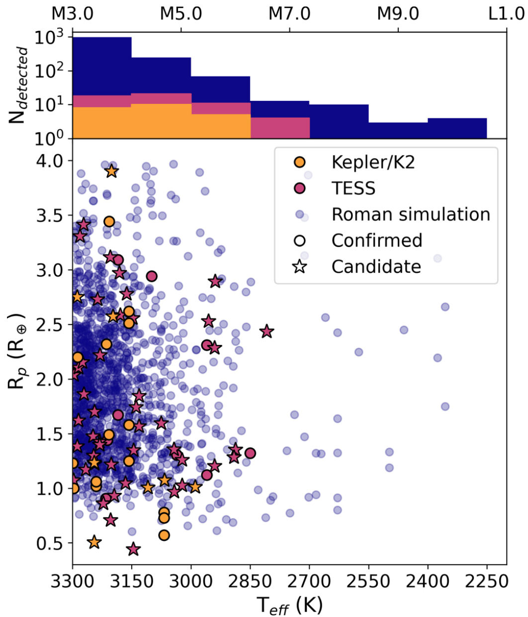
Figure 8. from Patrick Tamburo et al 2023 Astron. J. 165 doi:10.3847/1538-3881/acd1de https://dx.doi.org/10.3847/1538-3881/acd1de © 2023. The Author(s). Published by the American Astronomical Society.
