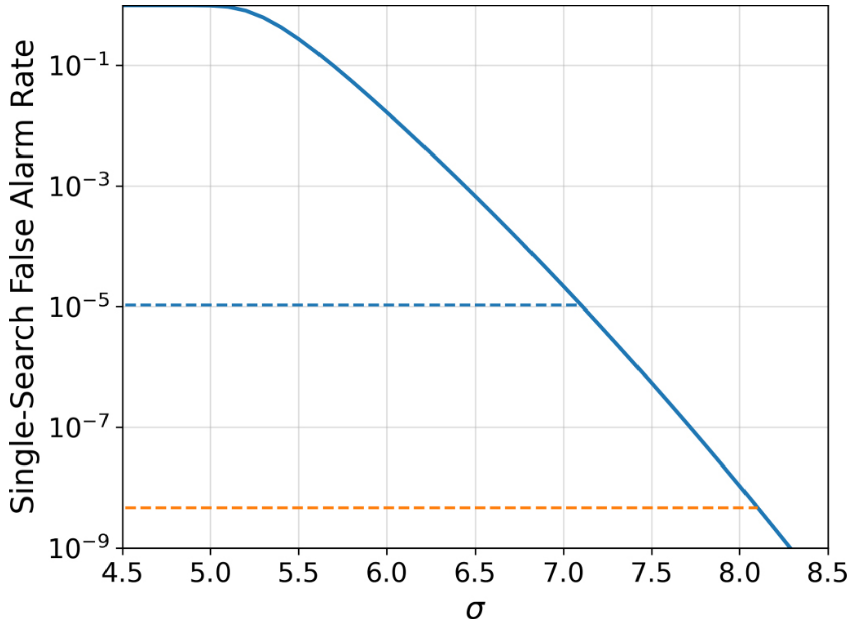
Figure 6. from Patrick Tamburo et al 2023 Astron. J. 165 doi:10.3847/1538-3881/acd1de https://dx.doi.org/10.3847/1538-3881/acd1de © 2023. The Author(s). Published by the American Astronomical Society.
