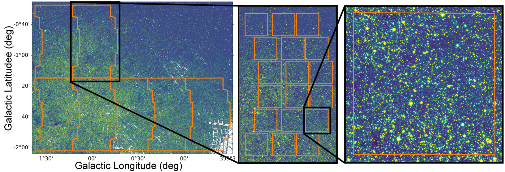
Figure 3. from Patrick Tamburo et al 2023 Astron. J. 165 doi:10.3847/1538-3881/acd1de https://dx.doi.org/10.3847/1538-3881/acd1de © 2023. The Author(s). Published by the American Astronomical Society.
