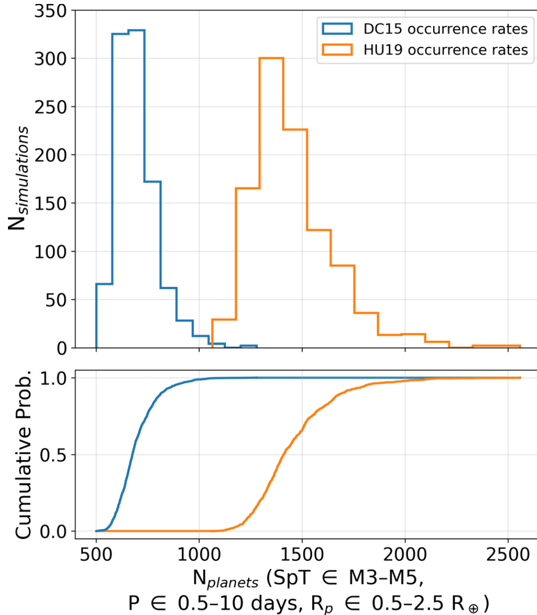
Figure 10. from Patrick Tamburo et al 2023 Astron. J. 165 doi:10.3847/1538-3881/acd1de https://dx.doi.org/10.3847/1538-3881/acd1de © 2023. The Author(s). Published by the American Astronomical Society.
